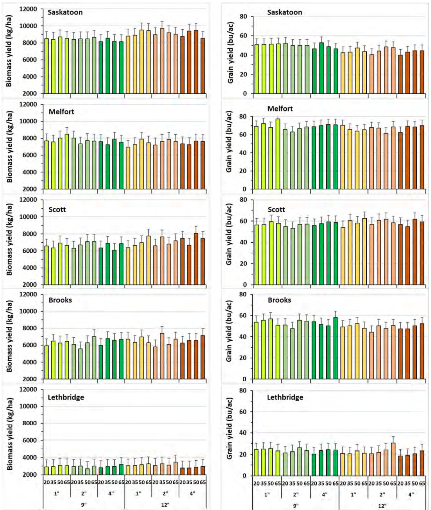
Fig. 23. Effect of increasing rate of seed-placed P fertilizer at various row spacing and opener width on biomass yield and grain yield at various locations averaged over 2018 and 2019 seasons. Error bars denote Tukey's HSD at \alpha = 0.05 level of significance.
