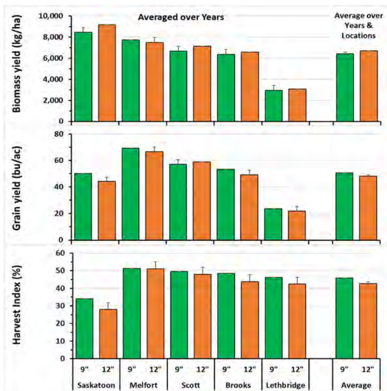
Fig. 17. Effect of row spacing on biomass yield, grain yield and harvest index at various locations. Error bars denote Tukey's HSD at \alpha = 0.05 level of significance.
