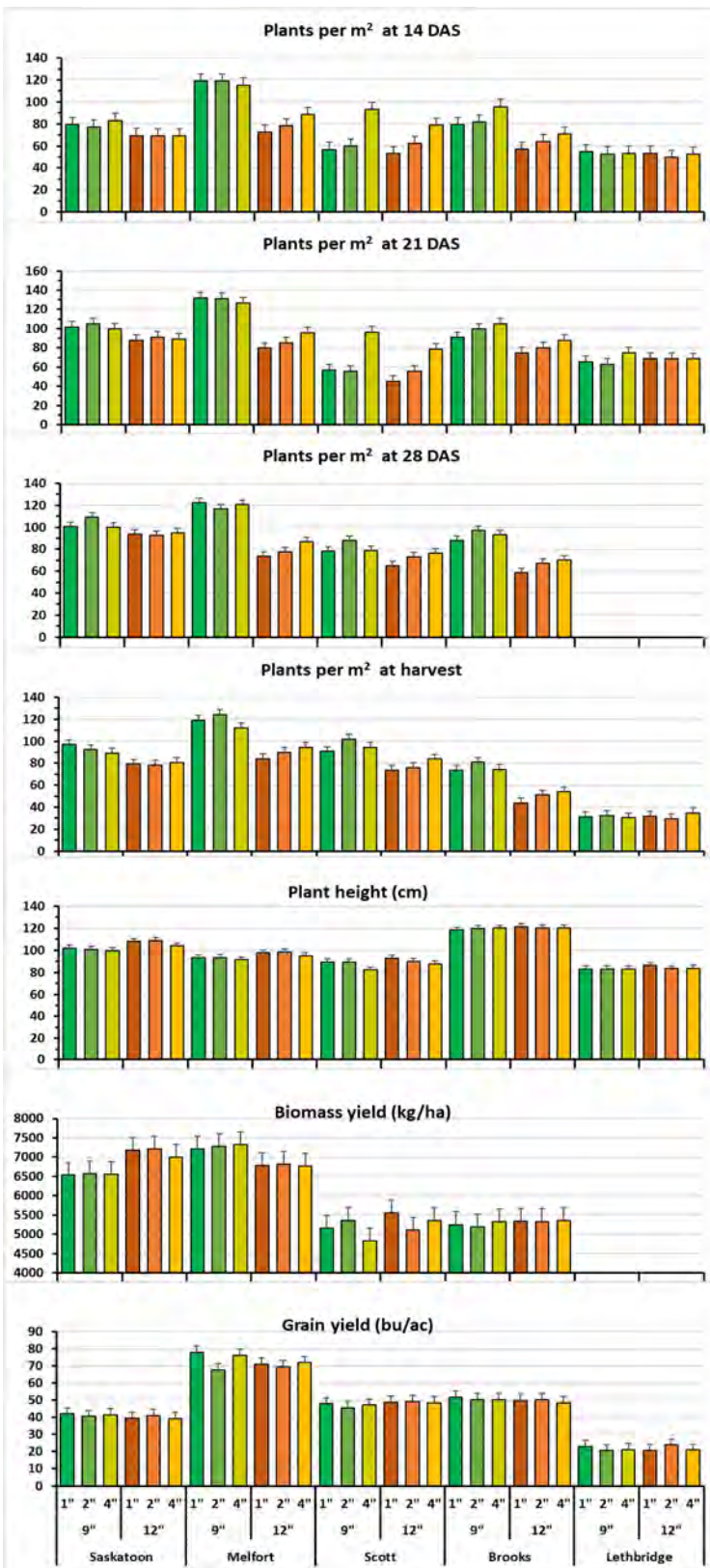
Fig. 9 . Interaction effect of row spacing and opener width on plant density, plant height and grain yield of canola at combined over locations in 2018. Error bars denote Tukey's HSD at \alpha = 0.05 level of significance.
