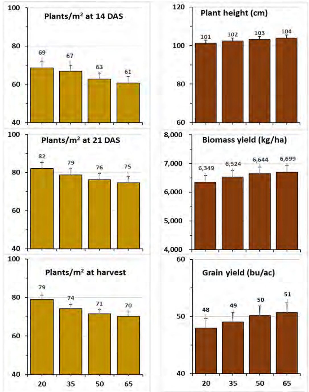
Fig. 21. Effect of seed-placed phosphorus rate on plant density, plant height, biomass yield and grain yield. Error bars denote Tukey's HSD at \alpha = 0.05 level of significance.
