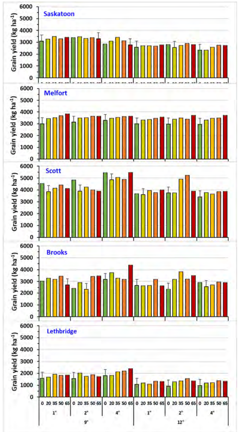
Fig. 15. Interaction effect of row spacing, opener width and rate of phosphorus on grain yield of canola in 2019. Error bars denote Tukey's HSD at \alpha = 0.05 level of significance.
