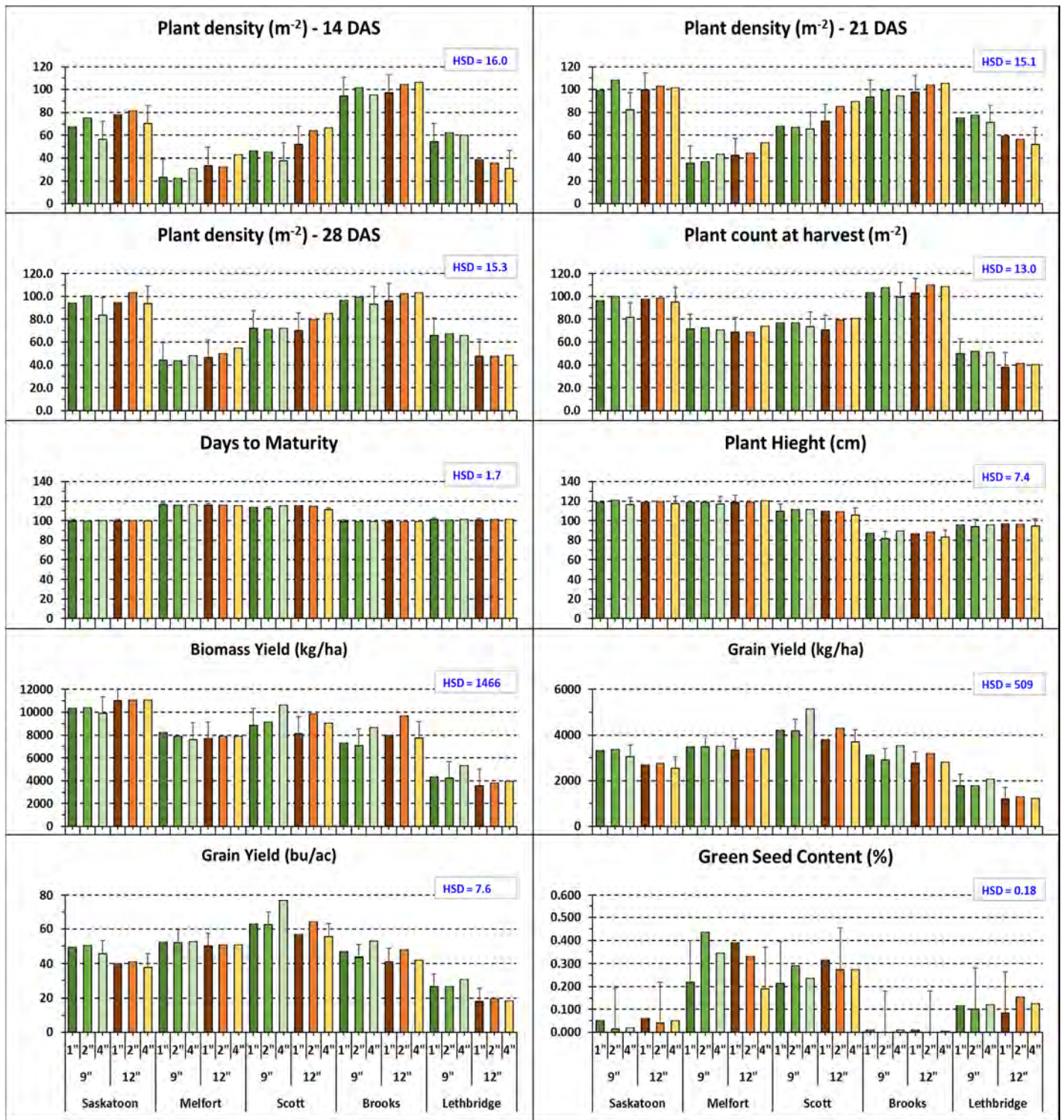
Fig. 13. Interaction effect of row spacing and opener width on plant density, plant height and grain yield of canola at combined over locations in 2019. Error bars denote Tukey's HSD at \alpha = 0.05 level of significance.
